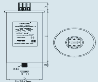
Mounting draw
